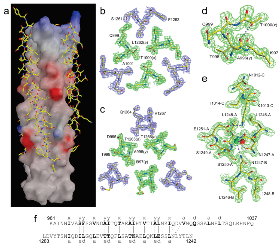
FIGURE 5: Interhelical packing interactions in the N57/C42 complex. (a) Surface properties of the N57 coiled-coil trimer with the C42 chains drawn as an atomic model. The solvent-accessible surface is colored according to the local electrostatic potential, ranging from +12 V in dark blue (most positive) to −19 V in deep red (most negative). (b) Cross-section of the N57(L10)/C42 trimer showing that side-chain packing of Leu1262 (blue) at the a position of C42 against Thr1000 (green) at the x position of N57. The 2F_o - F_c electron density map (contoured at 1.5 \sigma ) is shown with the refined molecular model. (c) Cross-section of the N57(L10)/C42 trimer showing side-chain packing of Thr1265 and Thr1266 (blue) at the d and e positions of C42 against Ala996 and Ile997 (green) at the y positions of N57. (d) A buried hydrogen-bonding interaction between the side chain of Thr1000 ( x ) and the carbonyl group of Ala996 ( y ). Hydrogen bonds are shown as purple dotted lines. (e) A buried interhelical salt-bridge between Glu1251 ( d ) and Lys1013; the carboxylate group coordinates to a bound sodium ion (pink sphere). (f) Schematic representation of packing interactions between two N57 helices and a C42 helix. Packing interactions between residues at positions x and y of N57 and residues at positions a , d , and e of C42 are indicated by solid lines. The side chain of Leu1246 of C42 packs against Ile1014 ( x ) and Val1018 ( a ) of N57 (indicated by dotted lines).
