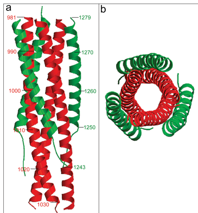
FIGURE 3: Crystal structure of the HCoV-NL63 N57(L10)C42 complex. (a) Lateral view of the N57(L10)C42 trimer. The N57 helices are shown in red and the C42 helices in green. The N termini of the N57 helices point toward the top of the page, and those of the C42 helices point toward the bottom. Residues are numbered according to their position in the HCoV-NL63 S sequence. (b) Axial view of the N57(L10)C42 trimer. The view is from the N termini of the N57 helices looking down the 3-fold axis of the trimer.
